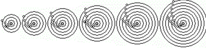
Figure 1: Expanding Cosmos
