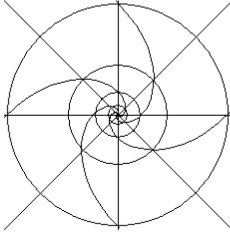
Figure 5: Logarithmic spirals
